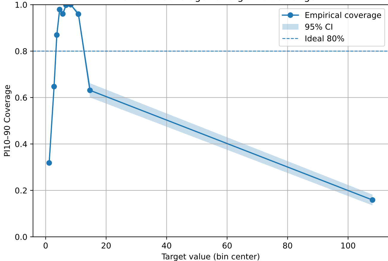
BPIC20DD: Coverage vs Target Value Range
